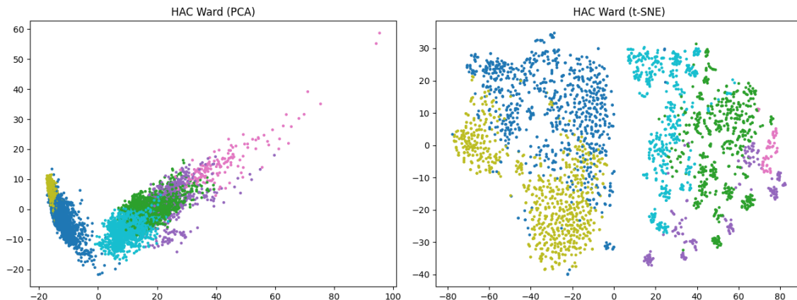
Figure 7: Hierarchical clustering with Ward linkage ( n\_clusters = 6 ) visualized with PCA (left) and t-SNE (right)
