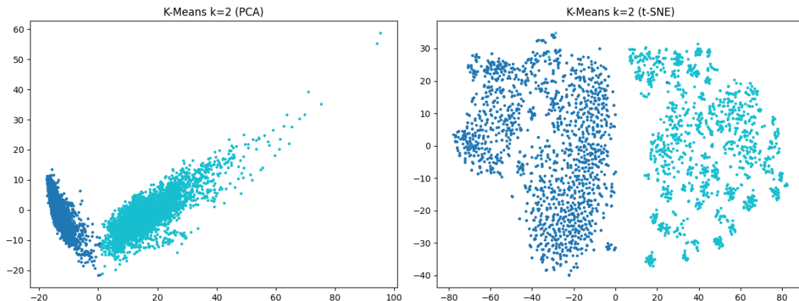
Figure 4: K-Means clusters for k = 2 visualized with PCA (left) and t-SNE (right)
